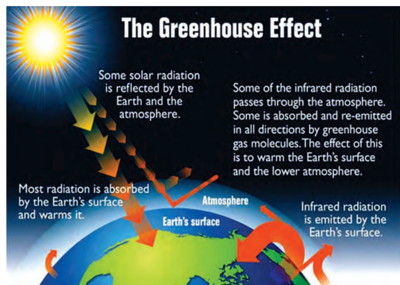
Figure 1. A schematic diagram of greenhouse effect
